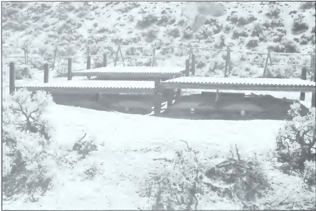
Photo 1. Northern guzzler details. Front aprons share three central uprights; rear apron shares uprights with one front apron. Gutter is in place and connected to tanks. Tops of tanks and sewer and drainpipe (S& D) protecting gate valves are visible.
